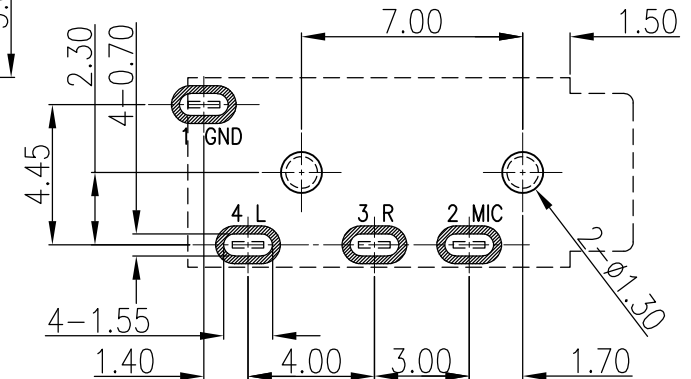
P.C.B LAYOUT BOTTOM VIEW (for reference only)
