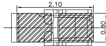
P.C.B LAYOUT TOLERANCE:±0.05
