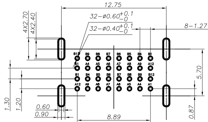
USB CF 16PIN RECOMMENDED PCB LAYOUT(TOP VIEW) THICKNESS 1.6MM;DEFAULT TOLERANCE:±0.05,SCALE 2:1
