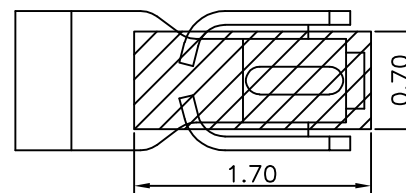
P.C.B LAYOUT TOLERANCE:±0.05
