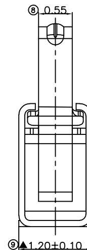
P.C.B LAYOUT TOLERANCE:±0.05
