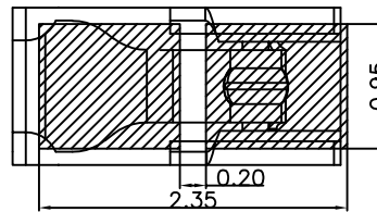
P.C.B LAYOUT TOLERANCE:±0.05
