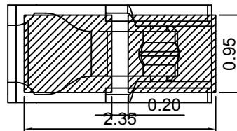
P.C.B LAYOUT TOLERANCE:±0.05
