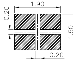
P.C.B LAYOUT TOLERANCE:±0.05
