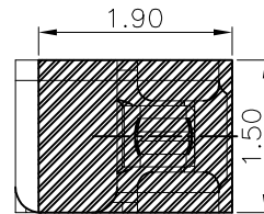
P.C.B LAYOUT TOLERANCE:±0.05
